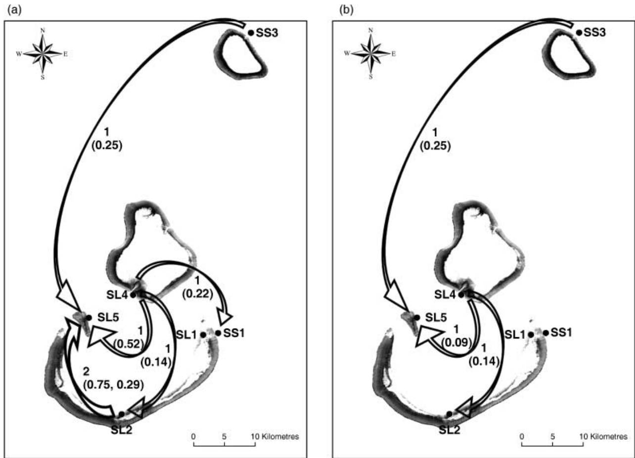
Fig. 5 Migration patterns at Scott Reef as inferred by GENECLASS 2 showing dispersal direction and numbers of immigrants that were excluded from their sampling site at P \leq 0.05 (a) or P \leq 0.01 (b) but were also assigned to source sites when P \geq 0.1 (a) or P \geq 0.05 . (b) Figures in brackets indicate probability that each individual originated from its assigned site.
