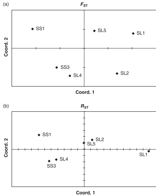
Fig. 4 Plots of principal coordinate analysis calculated in GENALEX from standardized distance matrix of Seriatopora hystrix sites at Scott Reef. (a) Pairwise F_{ST} estimates between sites: first two axes explain 95.93% of variation. (b) Pairwise R_{ST} estimates between sites: first two axes explain 98.16% of variation.
